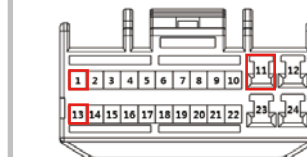
커넥터 B(Wire in view)
